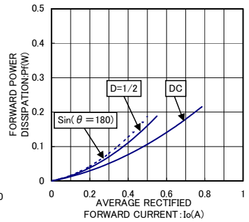
Io-Pf CHARACTERISTICS
